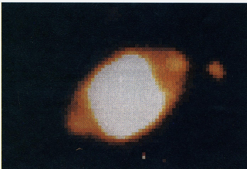
Figure 2: A 10-min H\alpha exposure of 19+501. Seeing is 0.8 arcsec FWHM. Note the faint, high excitation blobs.
