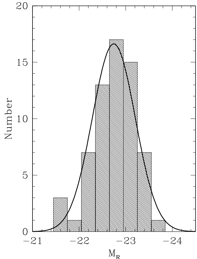
FIG. 2.—Distribution of the host galaxy absolute magnitude M_R for objects of group A. The solid line represents a Gaussian fit to the distribution (mean M_R = -22.8 , \sigma = 0.5 ).
