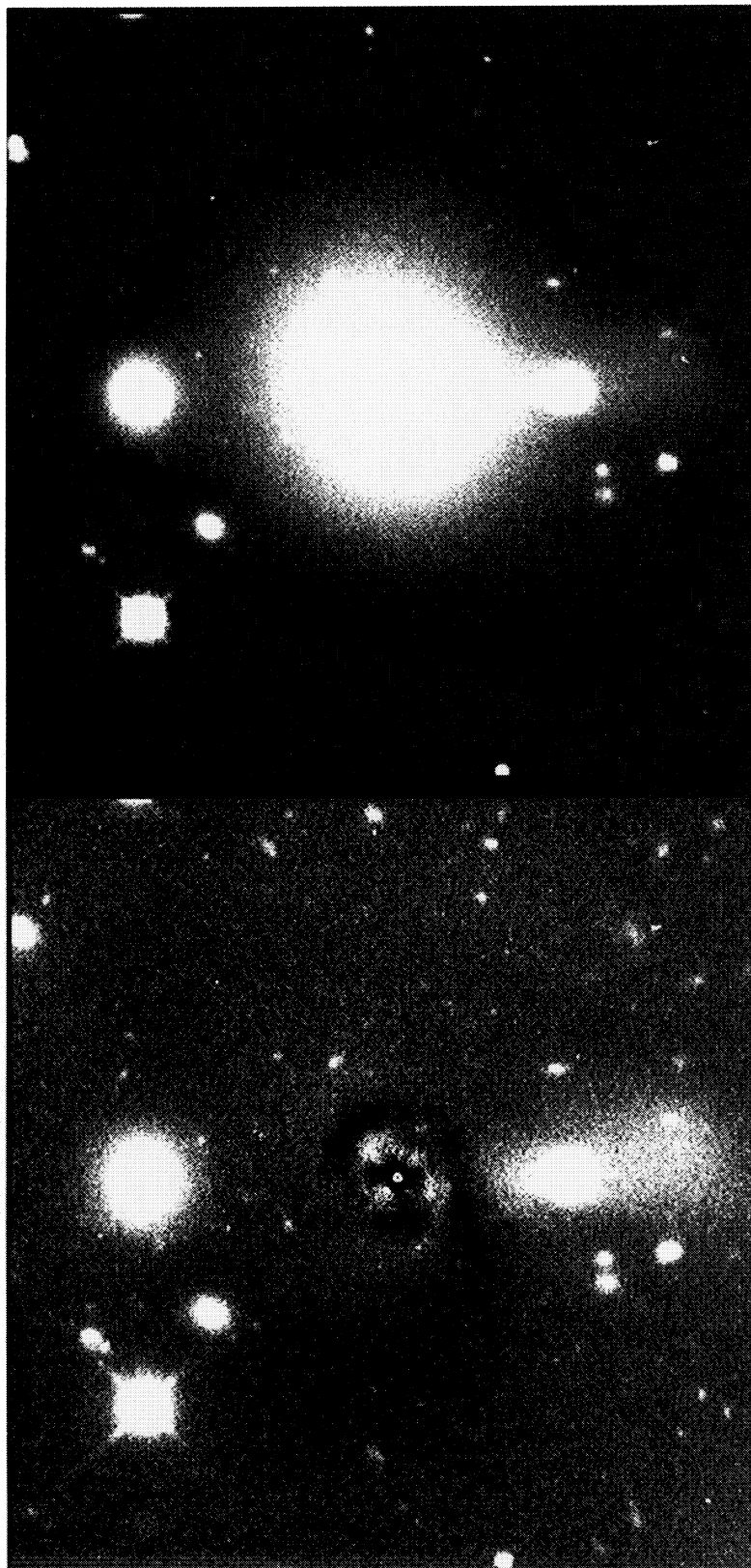
FIG. 2.—The host galaxy of the BL Lac object PKS 0548 – 322 ( top panel ), with the companion galaxies G6 and G7 ( left and right ; see text ). North is at the top, and east is to the left. The companion galaxies, together with the low surface brightness emission west of galaxy G7, are clearly visible after subtraction of a model including the host galaxy and the BL Lac nucleus ( lower panel ). The dark “spiral-shaped” feature around the nucleus is an artifact due to the subtraction of the model.
